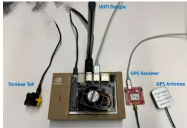
Figure 2: Hardware Platform with Wi-Fi dongle, GPS receiver, and Terabeer ToF
